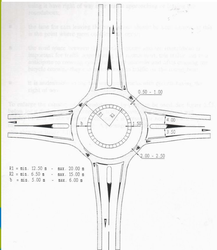
Figure 5.12: Roundabout with cycle lane and physical separation (hedgehogs).
